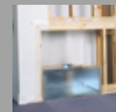
Zero Clearance Box positioned in framework on 50mm Hebel Blocks
